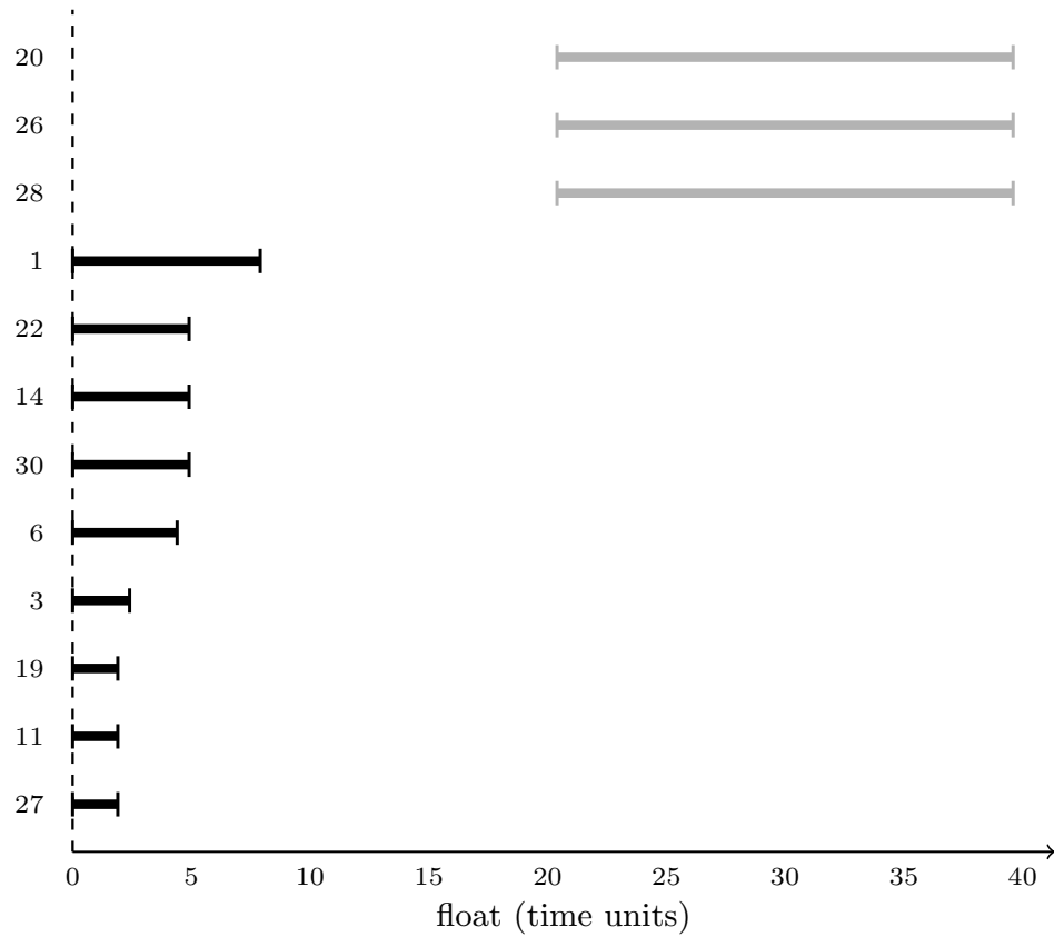
Figure 4: Exact float bounds on the water network with every duration at plus or minus 20 percent. Black bars are the nine possibly-critical stages, whose lower bounds reach zero. Grey bars are three of the 23 stages whose floats stay provably positive everywhere in the uncertainty box.
