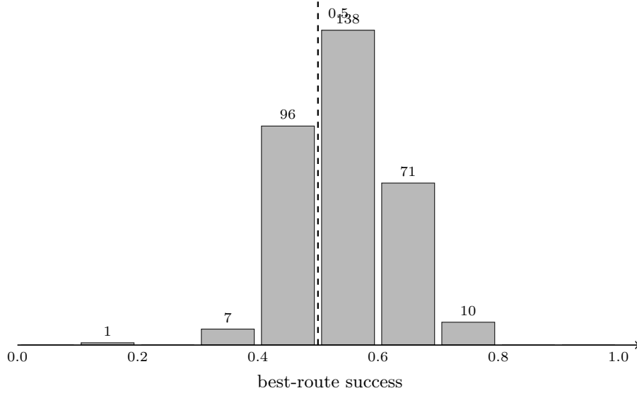
Figure 5: Best-route success across the 323 drone destinations. Left of the dashed line at 0.5 lie the 104 destinations that no single route serves reliably.
